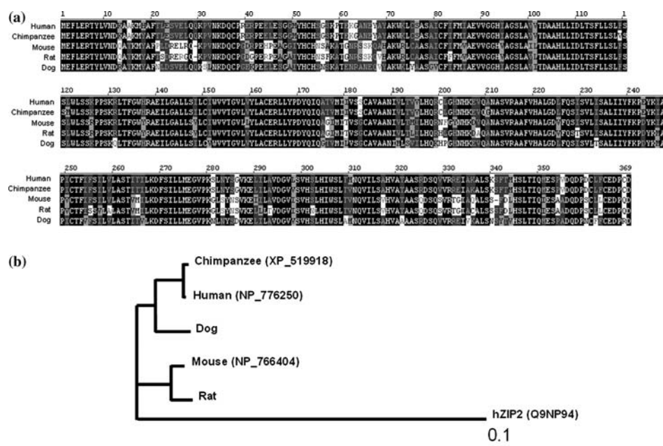
Figure 1. Alignment and phylogeny of ZnT-8 ortholog proteins. (a) Amino acid alignment of ZnT-8 protein sequences identified in Homo sapiens (human, NP_776250), Pan troglodytes (chimpanzee, XP_519918), Mus musculus (mouse, NP_766404), Rattus norvegicus (rat) and Canis familiaris (dog) were performed with ClustalW program. Black boxes correspond to conserved residues in all the sequences while grey and white boxes correspond to partially conserved residues. (b) For phylogenetic analysis ZnT-8 protein sequences were aligned using the clustalW program. Bootstrapping (2000 replicate sets) and calculation of the consensus tree were done with the DAMBE program. The scale of the branch length is given in amino acid substitutions per site.
